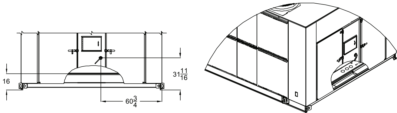
Figure 37. Electrical entry details/bottom view
