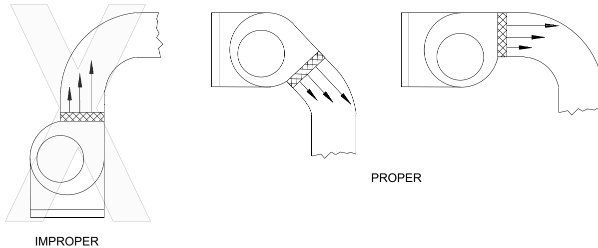
Figure 22. Duct design
