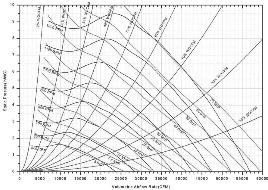
Figure 34. Return fan performance STANDARD CFM – 120-150 tons air-cool/128-162 tons evap-condensing (44")
