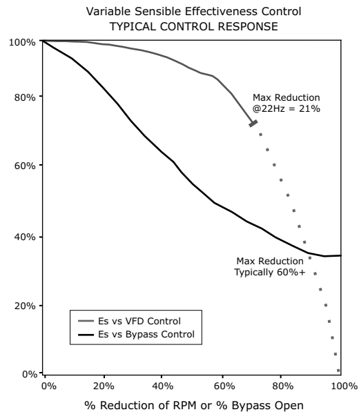
Figure 18. Variable sensible effectiveness control
