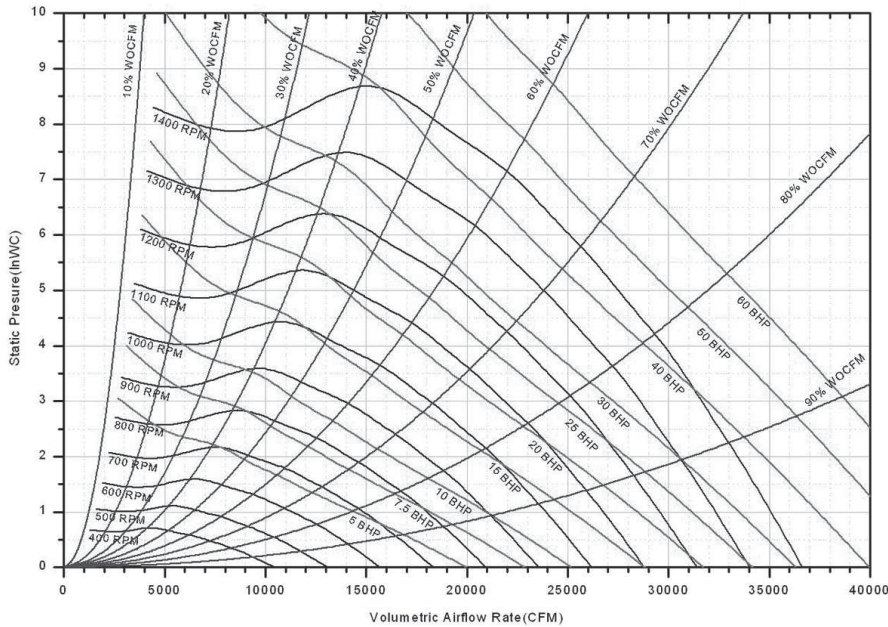
36.5" Return Fan Performance w/ Damper (6/21/05)
