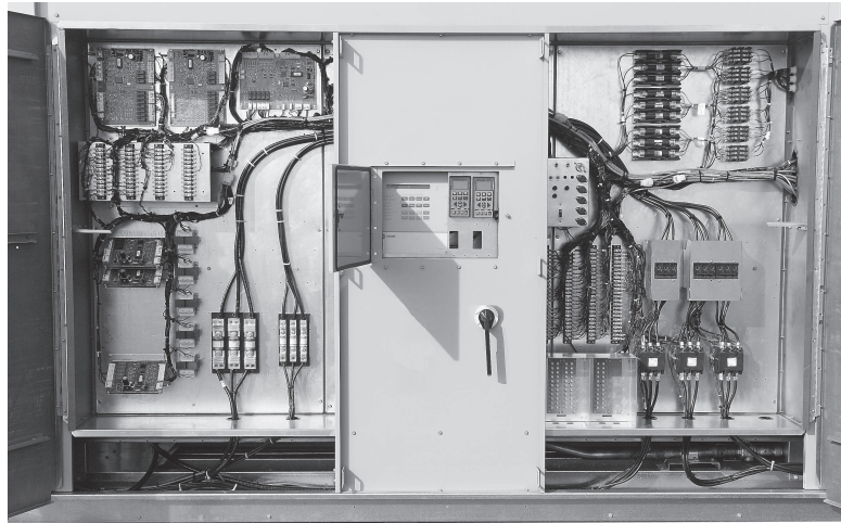
Figure 15. IntelliPak 2 control panel
