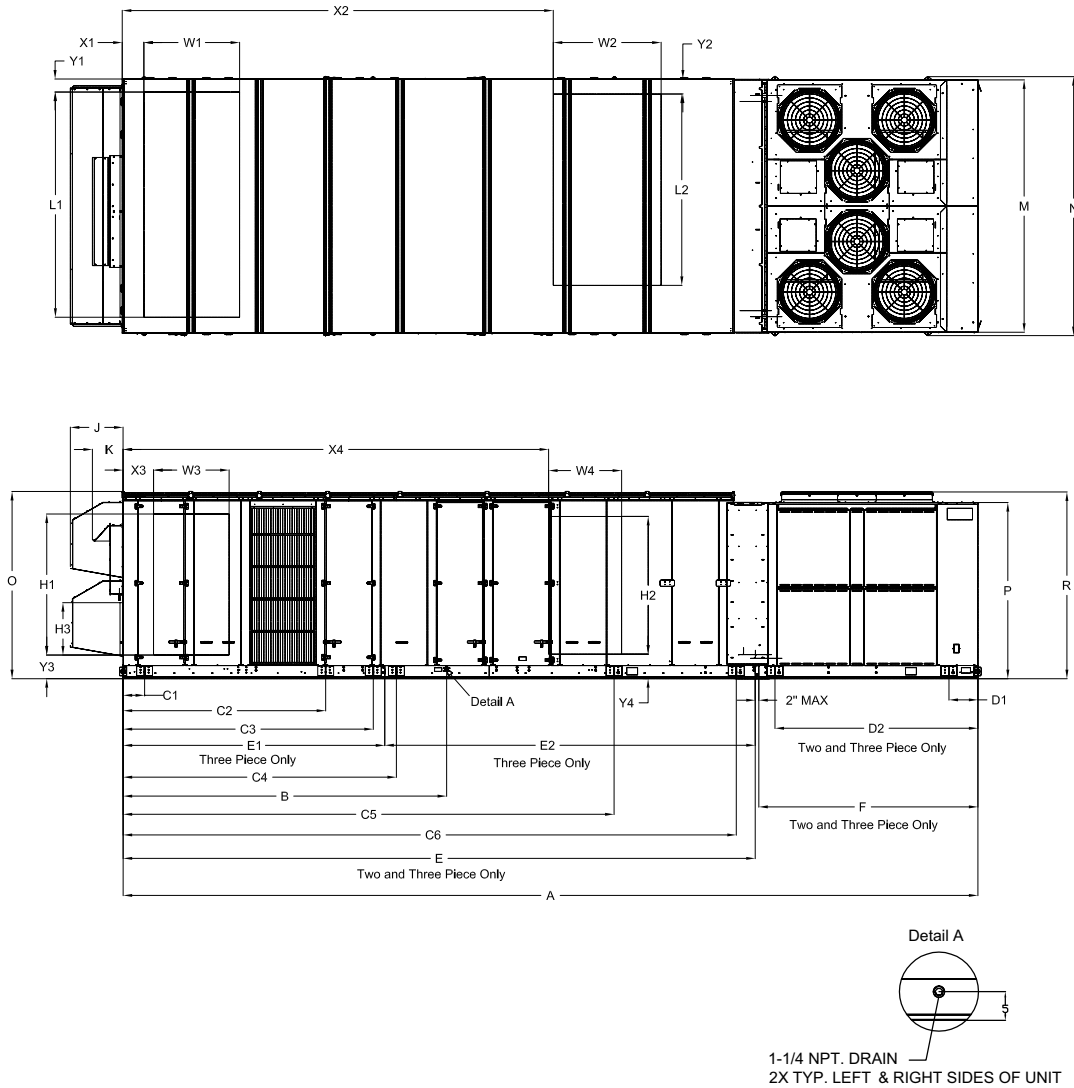
Figure 35. Unit top/left view
