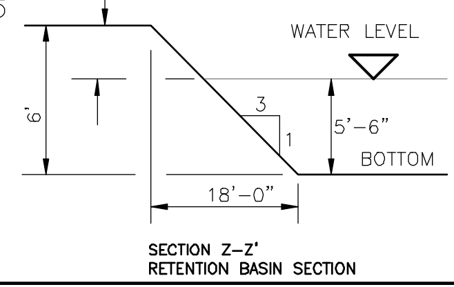
SECTION Z-Z' RETENTION BASIN SECTION
